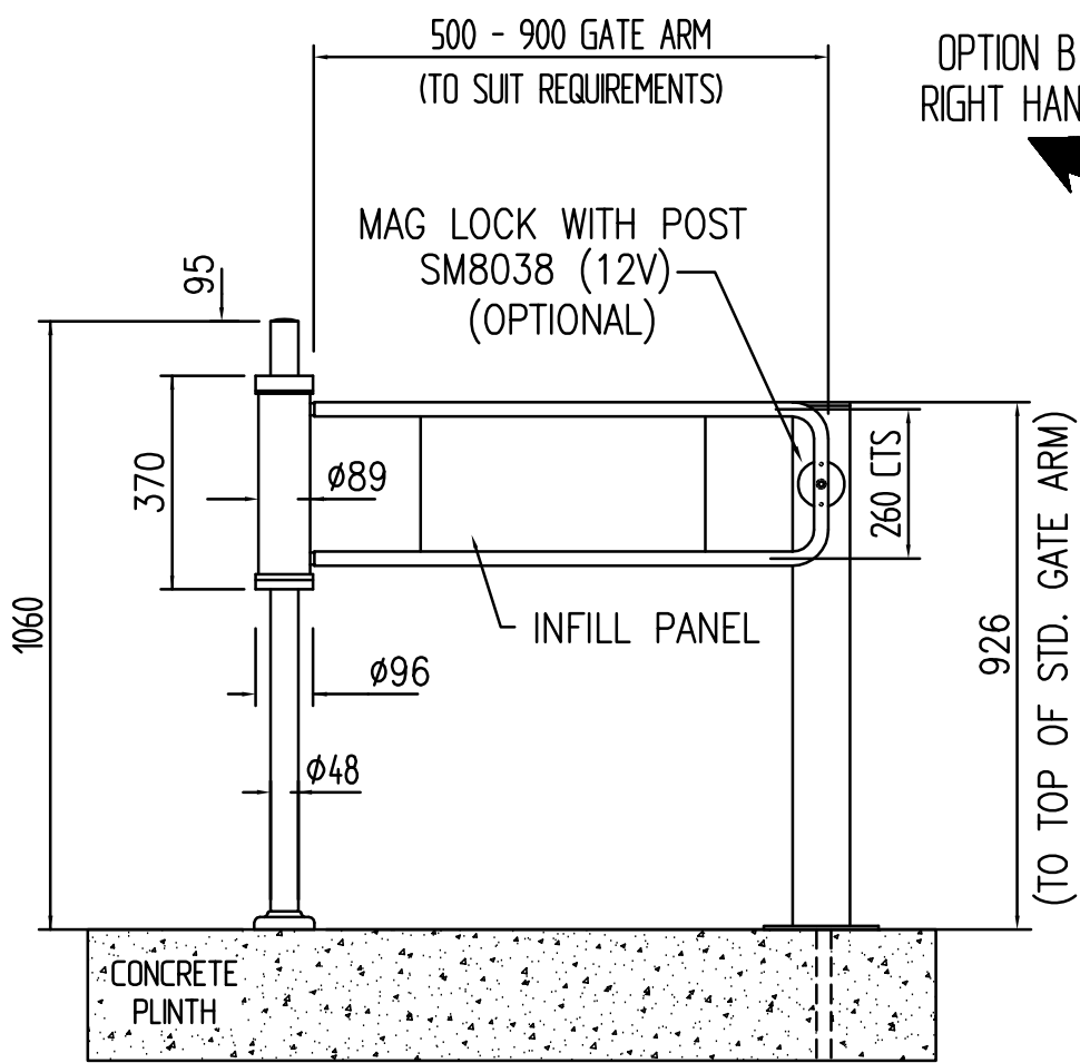
ELEVATION ON GATE
